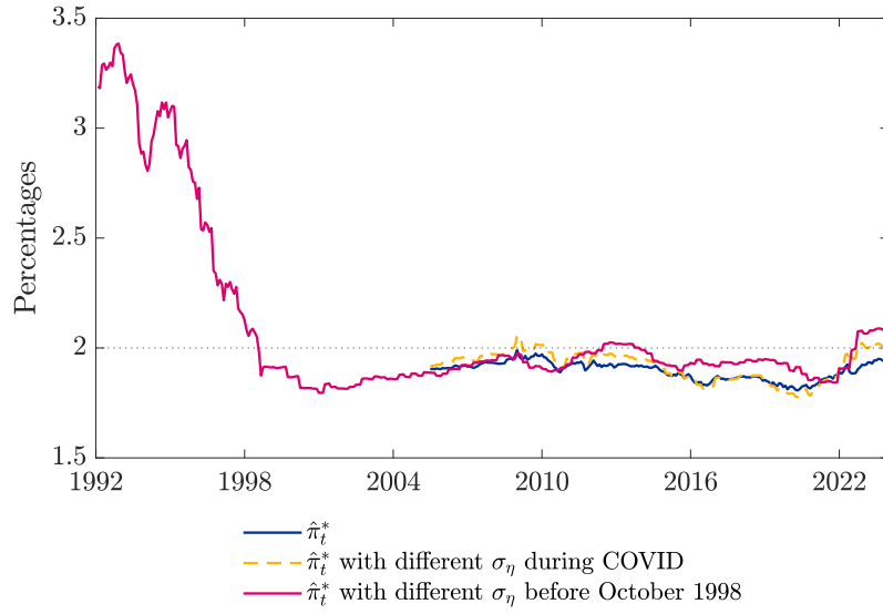
Figure 11: Estimated \pi_t^* with regime shifts.
